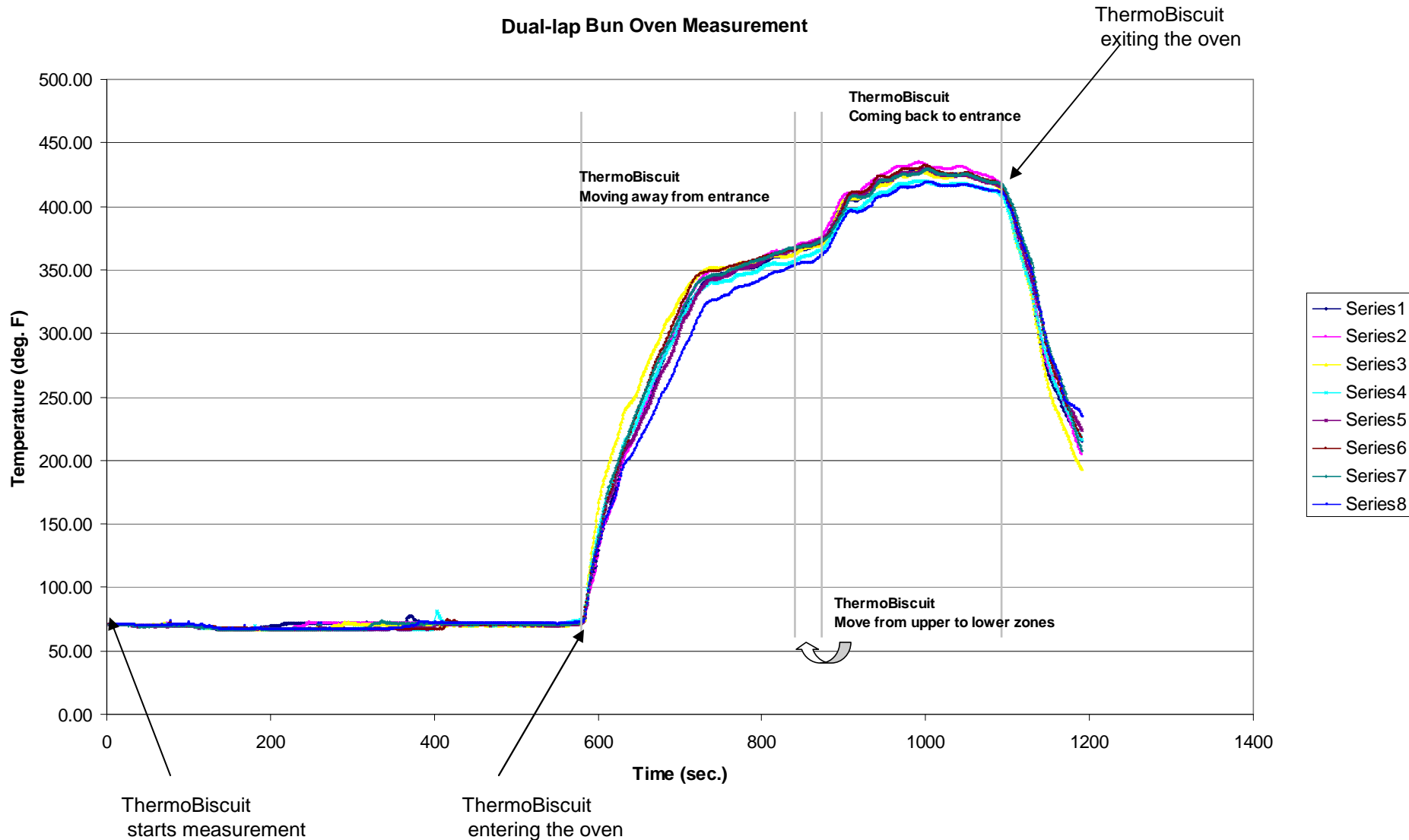
ThermoBiscuit travels through a bun oven and measure temperatures at the eight locations of a bun pan
